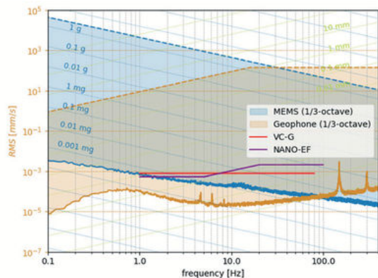
Geophone ( \pm 200 mm/s) - MEMS ( \pm 4 g) comparison
