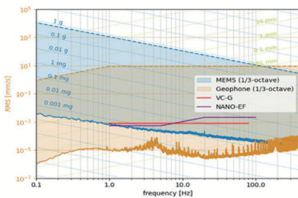
Geophone ( \pm 12.5 mm/s) - MEMS ( \pm 1 g) comparison
