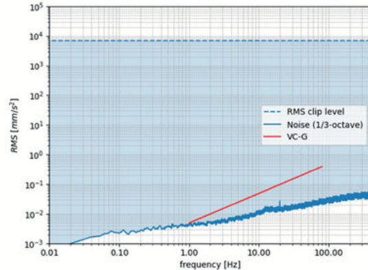
Geophone ( \pm 12.5 mm/s) - MEMS ( \pm 1 g) comparison
